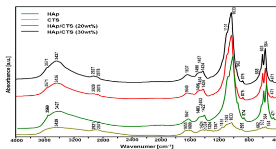
Fig. 2: FTIR spectra of chitosan, hydroxyapatite and HAp/CTS composites
