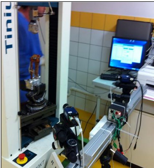
Fig. 1. Compression test.
