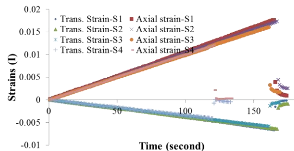
Fig. 1: The curve of axial-transversal strains (GR).
