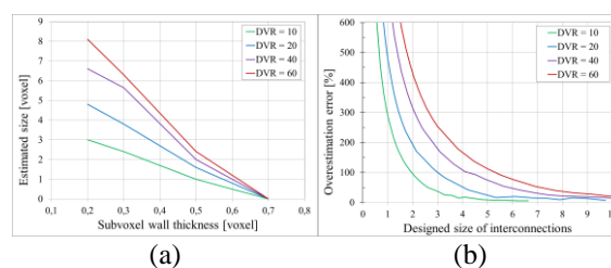
Fig. 2: (a) Estimated size of wrong connections. (b) Overestimation error of interconnections.
