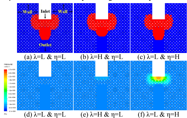
Fig. 1: Flow and pressure profiles of PMMA.
