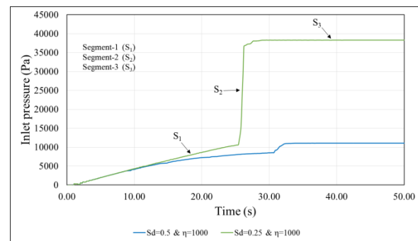
(c) Inlet pressure graph
