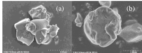
Fig.1: SEM of (a) Feed (b) milled for 60 minutes.
