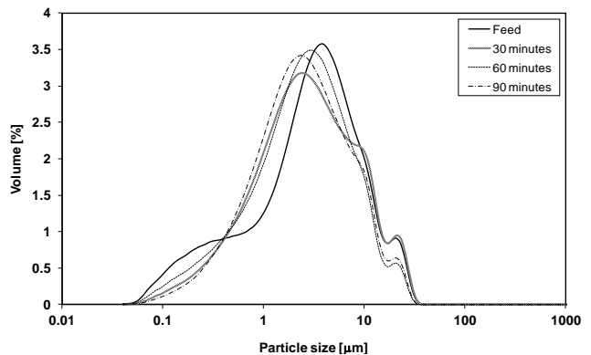
Fig.2: PSD of feed and milled powders.
