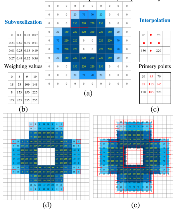
Fig. 1: (a) Original synthetic 2D object. (b) Subvoxelization and (c) interpolation steps in 4 original pixels (red in (a)). Gray levels of subpixels after (d) subvoxelization and (e) interpolation algorithms.
