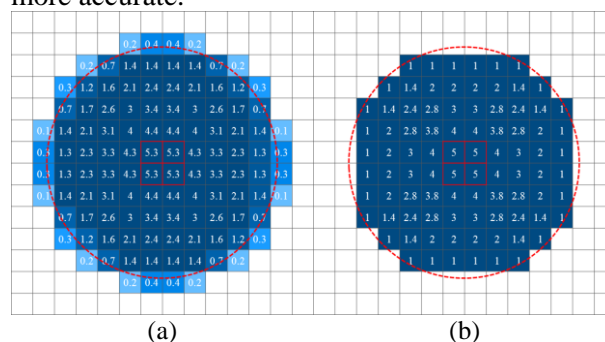
Fig. 1: (a) FDT and (b) DT of defined circular pore for DPR ≈ 10.
