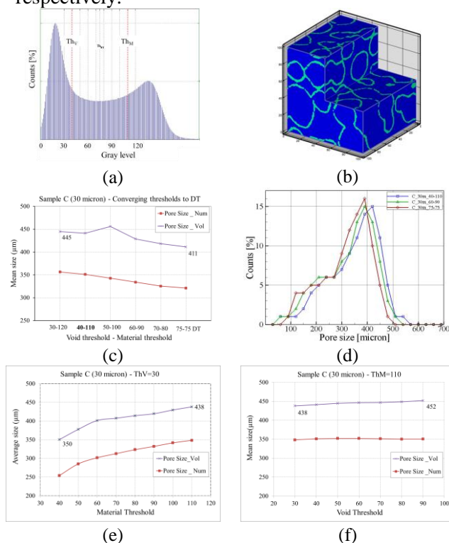
Fig. 1: (a) Gray level histogram. (b) Removed region via converging the thresholds. (c) Mean size and (d) size distributions of pores. Pore size sensitivity to variation of Th_M (e) and Th_V (f).
