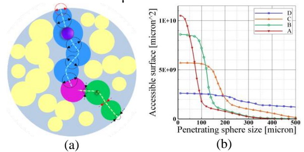
Fig. 1: (a) LPD of a pore via two paths. (b) Total accessible surface versus penetrating sphere sizes.
