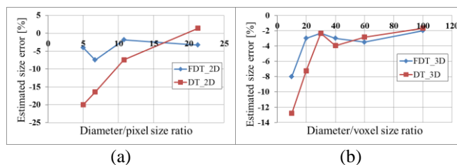
Fig. 2: Pore size errors by FDT versus DT in synthetic (a) 2D pores and (b) 3D pores.
