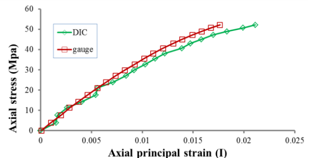
Fig. 3: The curves of principal stress versus strain.
