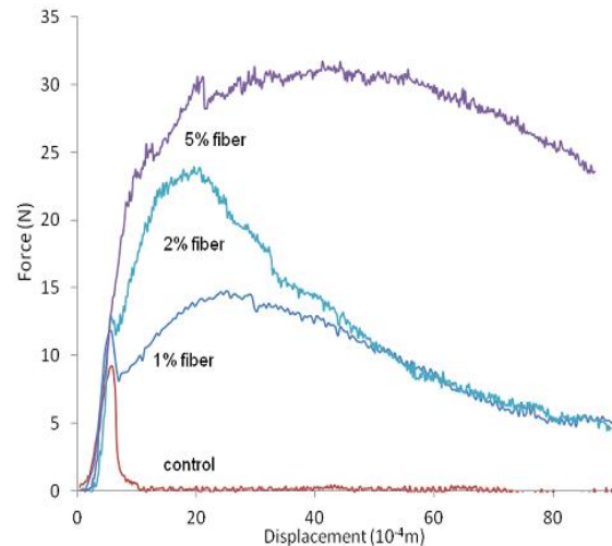
Fig1: 3 points bending tests on chevron notched specimens (8x8x36mm) of cotton FRCPC
