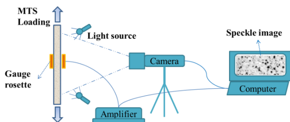
Fig. 1: DIC setup during axial tensile experiments.
